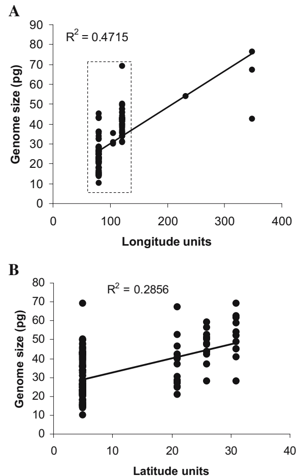
Figure 10. Regression analysis showing the relationship of genome size with longitude (A) and with latitude (B) in plethodontids. In both cases, longitude and latitude are expressed as a distance measurement. If only North American species are considered (box in graph A), the R^2 value increases to 0.58.
